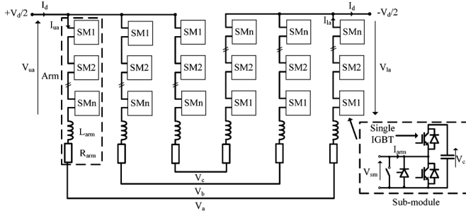
Fig. 1. Three-phase MMC.
