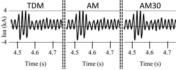
Fig. 15. Line-to-ground fault for phase A applied at 4.5 s.
